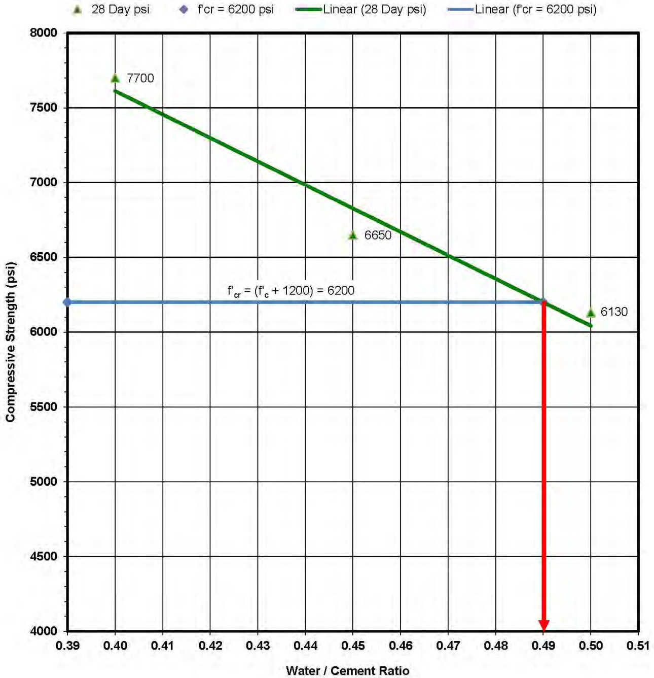
Compressive Strength vs. Water / Cement Ratio w/Line at f'_{cr} = 6200 psi
