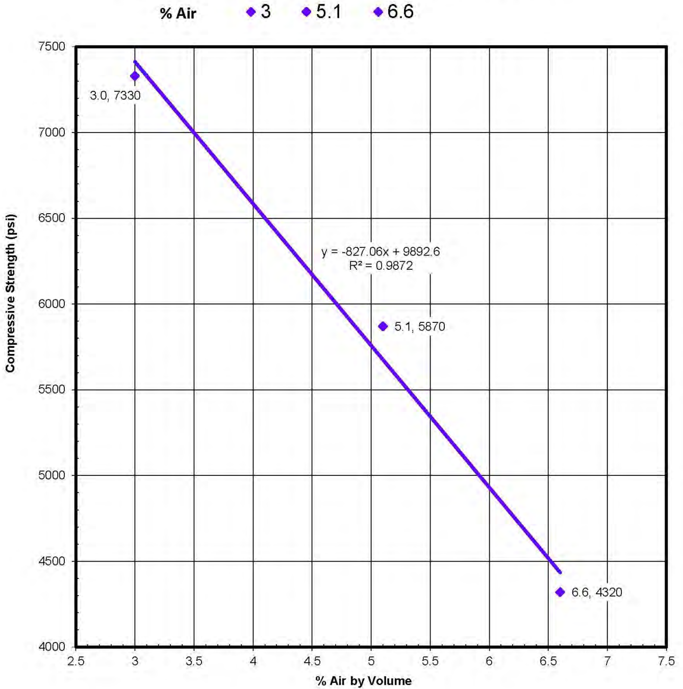
28 Day Compressive Strength vs % Air for 3 batches at w/c = 0.400
